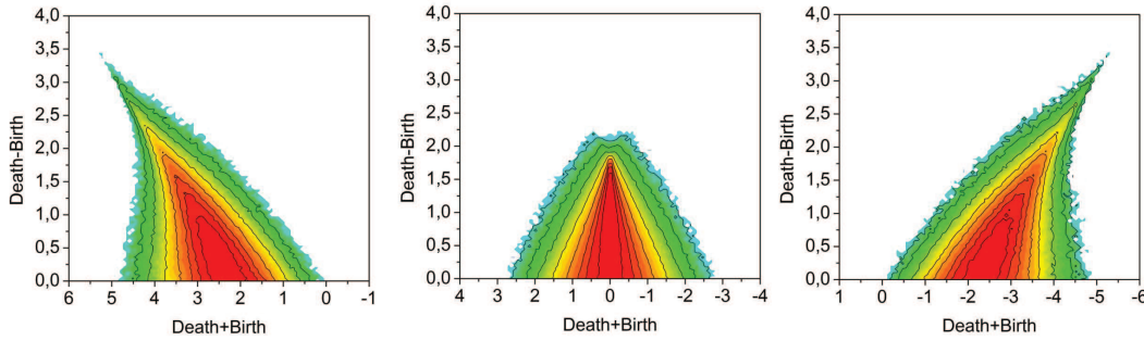
Figure 1. The empirical intensity plots computed by averaging the persistence diagrams of ten Gaussian random fields on the 3-torus. From left to right: the plots for 0-, 1-, 2-dimensional homology. (Pictures courtesy of Pratyush Pranav).
